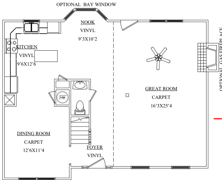
OPTIONAL LAYOUT (First Floor)
