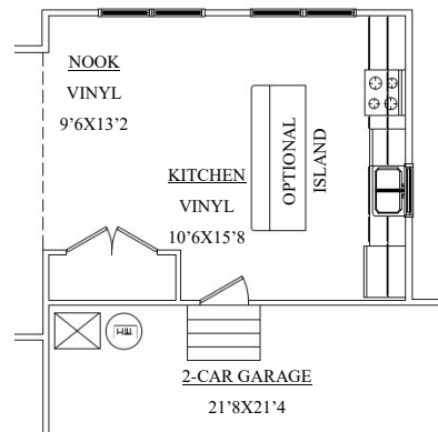
Optional Kitchen Layout 1
